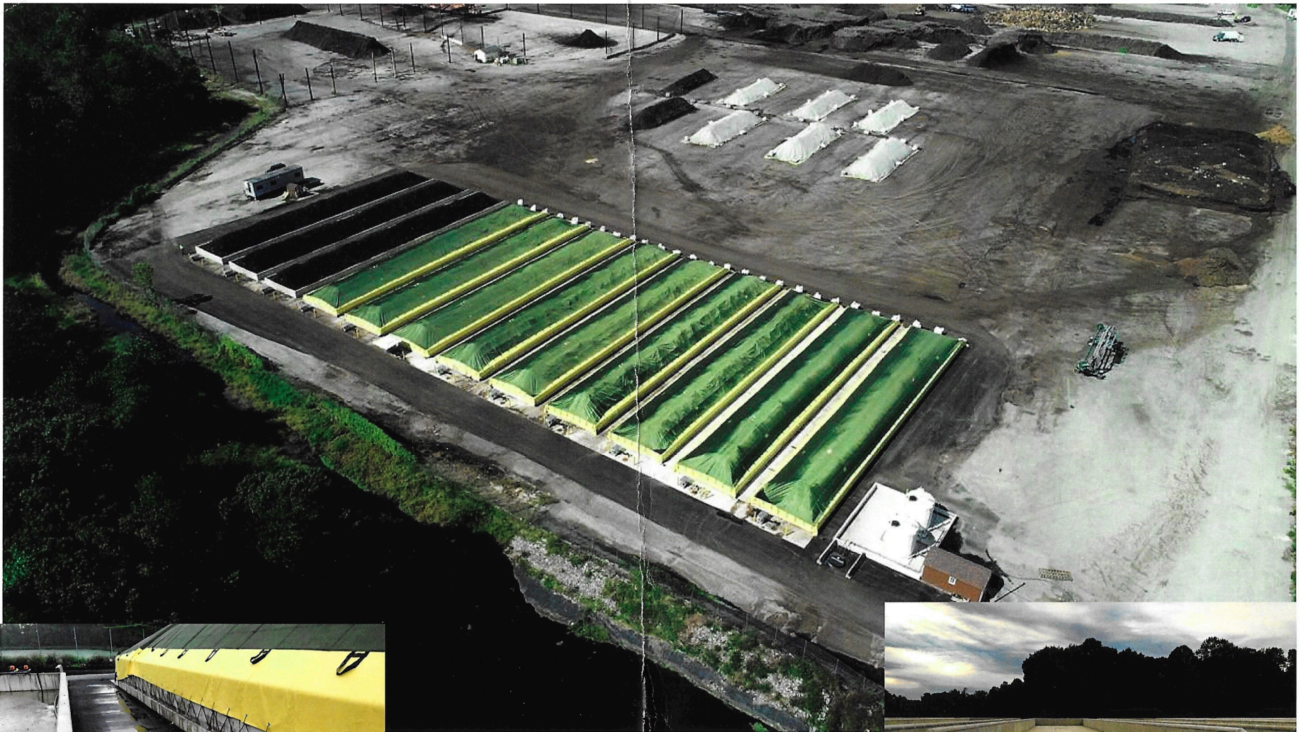
CASP SYSTEM: COVERED AERATED STATIC PILES - Feedstock is covered in a concrete bunker system process, creating a closed system that fully contains leachate and minimizes odors.
